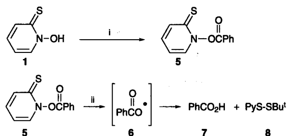
Scheme 1 Reagents and conditions: i, 1.1 equiv. of PhCOCl, 1.4 equiv. of pyridine, CH 2 Cl 2 , 0 °C, 1 h, 92%; ii, 5.0 equiv. of Bu t SH, CH 2 Cl 2 , hν (GE, 300 W, \lambda > 350 nm), 0 °C, 1 h, 92% (for 7 ) and 89% (for 8 )
