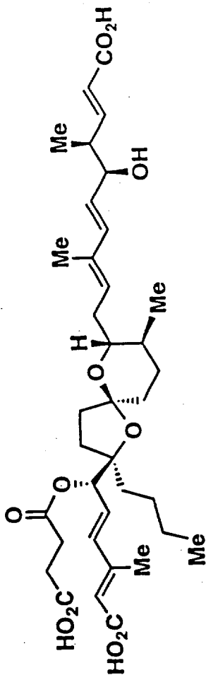
reveromycin B (2)
