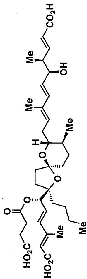
reveromycin B (2)
