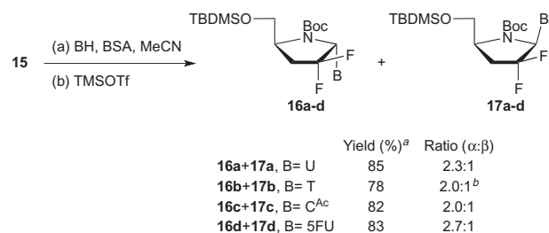
Scheme 2. Glycosylation of 15 with pyrimidines. Reagents and conditions: (a) 1 equiv 15 , 4 equiv base (BH = uracil, thymine, N 4 -acetylcytosine, and 5-fluorouracil), 6 equiv BSA, MeCN, 80^\circ\text{C} , 1 h; (b) 2.7 equiv TMSOTf, 0 – 80^\circ\text{C} , 30 min, 78–85% over two steps.
