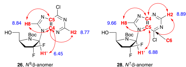
Figure 2. HMBC correlations of N^9 and N^7 regioisomers. In red are correlations mentioned in the text. The ^1\text{H} NMR values ( \delta ppm) are in blue.
