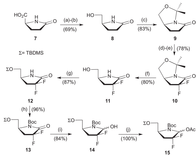
Scheme 1. Synthesis of 15 . Reagents and conditions: (a) 1 equiv \text{SOCl}_2 , MeOH, rt, 4 h; (b) 2 equiv \text{NaBH}_4 , EtOH, rt, 14 h; (c) 2,2-dimethoxypropane (solvent), 0.03 equiv CSA, reflux, 2 h; (d) 1.4 equiv ^i\text{Pr}_2\text{NH} , 1.2 equiv ^n\text{BuLi} , 1.4 equiv NFSI, THF, -78^\circ\text{C} ; (e) 1.4 equiv ^i\text{Pr}_2\text{NH} , 1.2 equiv ^n\text{BuLi} , 1.4 equiv NFSI, THF, -78^\circ\text{C} ; (f) AcOH/MeCN/ \text{H}_2\text{O} (14:3:3), 90^\circ\text{C} , 14 h; (g) 1.3 equiv TBDMSCl, 1.3 equiv imidazole, 0.1 equiv DMAP, \text{CH}_2\text{Cl}_2 , rt, 30 min; (h) 2 equiv \text{Boc}_2\text{O} , 1.3 equiv \text{Et}_3\text{N} , 1.1 equiv DMAP, \text{CH}_2\text{Cl}_2 , rt, 30 min; (i) 1.2 equiv \text{LiEt}_3\text{BH} , THF, -78^\circ\text{C} , 1 h; (j) 15 equiv \text{Ac}_2\text{O} , 30 equiv \text{Et}_3\text{N} , \text{CH}_2\text{Cl}_2 , rt, 30 min.
