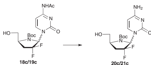
Scheme 4. Synthesis of 20c/21c . Reagents and conditions: \text{NH}_3 sat-MeOH, rt, 1 h, 82%.
