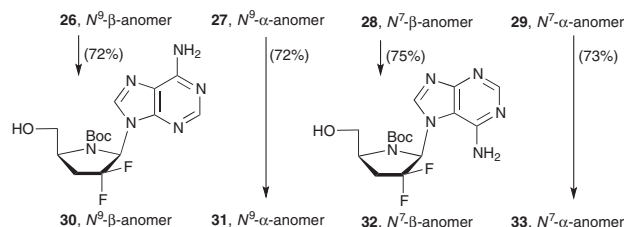
Scheme 6. Synthesis of adenine 4'-azanucleosides 30–33 . Reagents and conditions: \text{NH}_3 sat-MeOH, 100 °C, 3 h.
