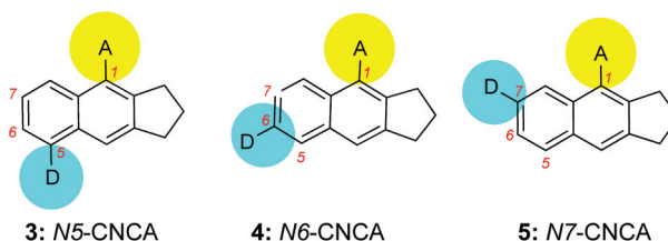
Fig. 4 Comparison of the relative position of donor (D, Me 2 N) and acceptor (A, CH=C(N)CO 2 TEGME) substituents in CNCA dyes. Placing the D and A groups in close proximity decreases their rotational ability thereby allowing emission from the planar excited state.
