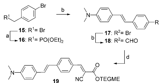
Scheme 4. Reagents and conditions: a) 1.0 equiv 15 , 15 equiv triethyl phosphite, 90 °C, 19 h, 98%; b) 1.0 equiv 16 , 1.0 equiv NaOMe, 1.0 equiv 6a , excess DMF, 25 °C, 24 h, 74%; c) 1.0 equiv 17 , 1.0 equiv n BuLi, 1.33 equiv DMF, THF, −78 °C, 60%; d) 1.0 equiv 18 , 1.1 equiv 7 , 0.1 equiv piperidine, THF, 50 °C, 21 h, 97%.
