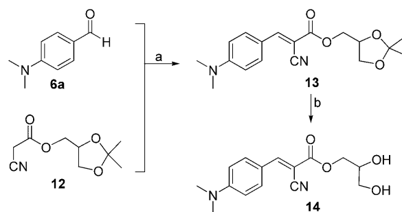
Scheme 3. Reagents and conditions: a) 1.0 equiv 6a , 1.1 equiv 12 , 0.1 equiv piperidine, THF, 50 °C, 21 h, 91%; b) 1.5 mmol 13 , 0.10 g DOWEX-H + , THF/CH 3 OH (1:1), 25 °C, 20 h, 75%.
