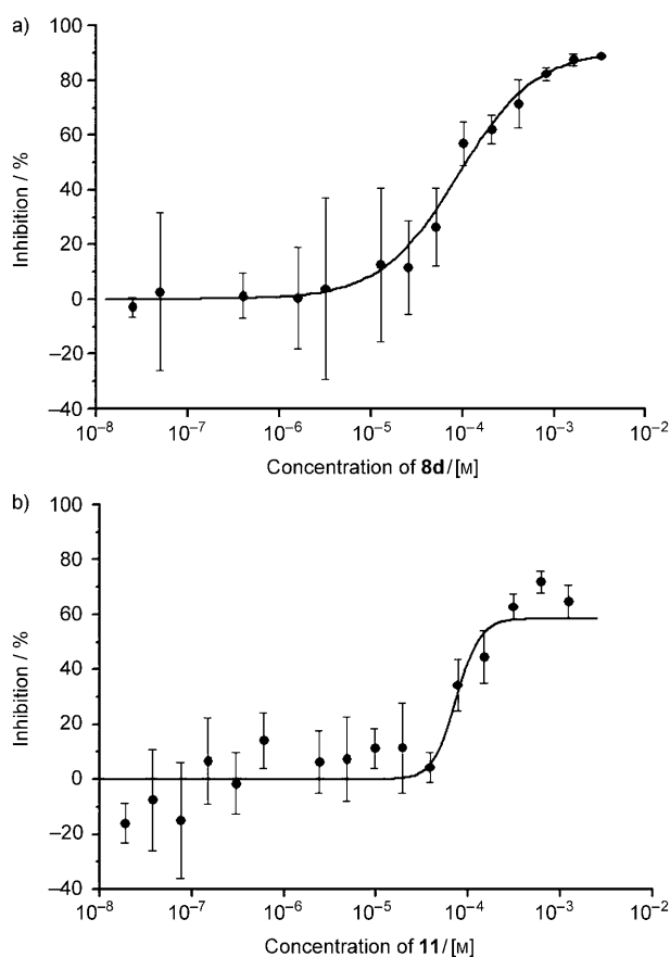
Figure 5. Inhibition of IgG-A \beta interactions with probes a) 8d ( I_{\max} = 91\% , IC_{50} = 91 \mu\text{M} ) and b) 11 ( I_{\max} = 58\% , IC_{50} = 74 \mu\text{M} ).
