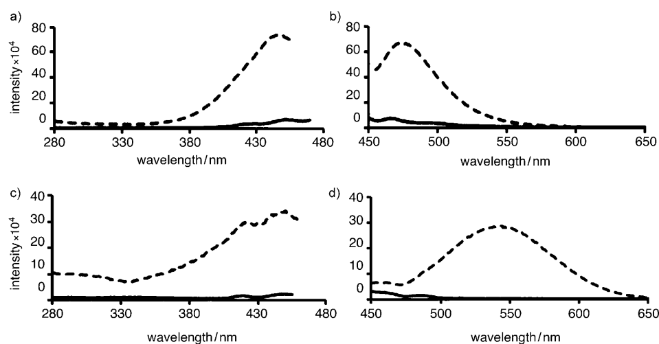
Figure 3. Fluorescence excitation (a, c) and emission spectra (b, d) of probes 8d (a, b) and 11 (c, d) in aqueous PBS solution (—) and in the presence of aggregated A \beta peptide (---).
