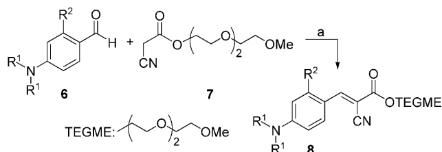
Scheme 1. Reagents and conditions: a) 1.0 equiv 6 , 1.1 equiv 7 , 0.1 equiv piperidine, THF, 50 °C, 21 h.
