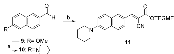
Scheme 2. Reagents and conditions: a) 8.0 equiv piperidine in benzene/HMPA: 1/1, 0 °C, 8.0 equiv n BuLi, 0 °C, 15 min, then 1.0 equiv 9 , 25 °C, 12 h, 35%; b) 1.0 equiv 10 , 1.1 equiv 7 , 0.1 equiv piperidine, THF, 50 °C, 21 h, 82%.
