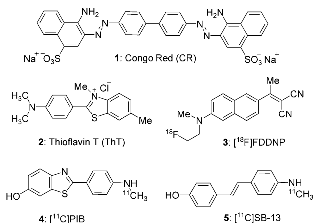
Figure 1. Structures of selected amyloid imaging reagents.
