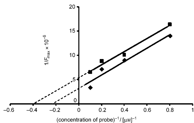
Figure 4. Determination of the apparent binding constant ( K_d ) of probes 8d (◆; R^2 = 0.95 ) and 11 (■; R^2 = 0.98 ) to preaggregated A \beta peptide.
